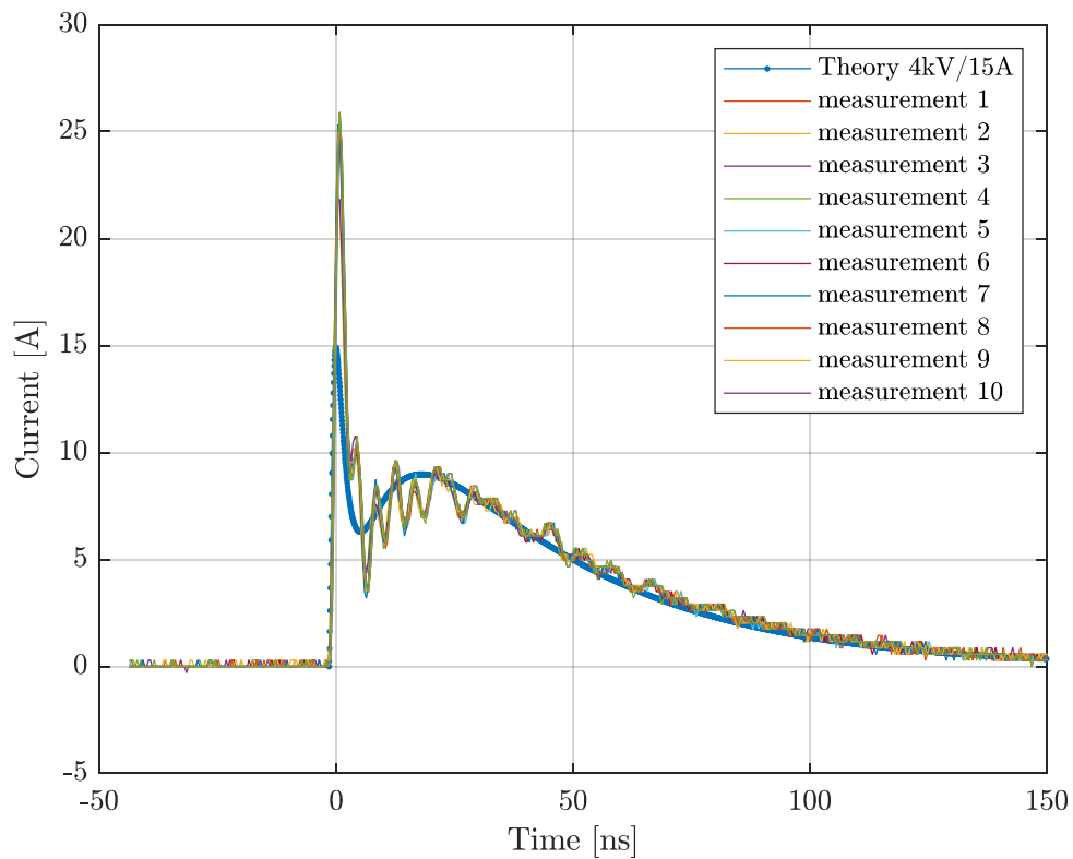
Figure 7. Measured results for shaper #7b (round edges).
