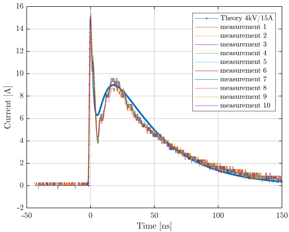
Figure 5. Measured results for shaper #1.
