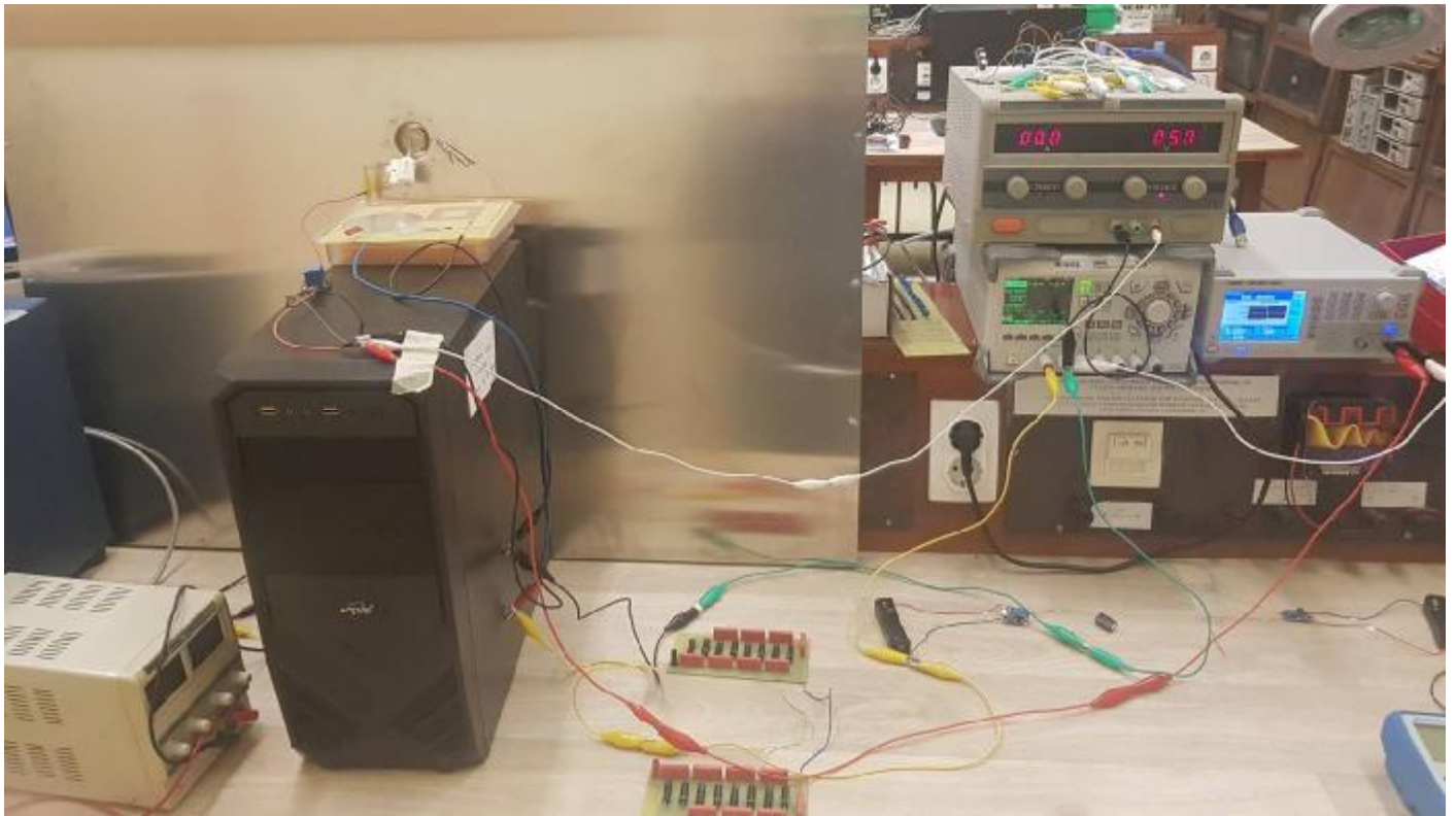
Figure 4. Measurement system for shaper response.
